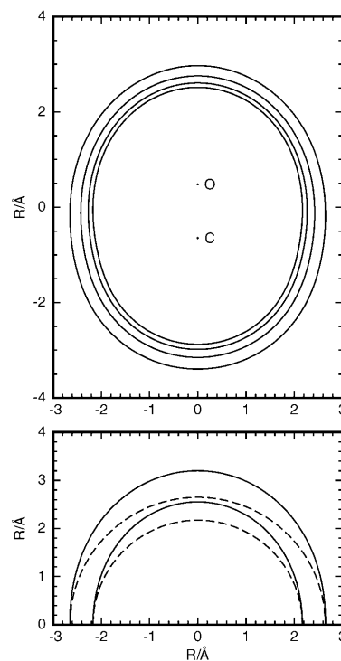
Figure 5. Top: repulsive-wall contours of the H 2 -orientation-averaged Jankowski-Szalewicz potential. From outermost to innermost the interaction energies are 6.5, 16.7, 30.2, and 43.0 kJ mol -1 . Bottom: hard-shell interactions as used for modelling of interactions between D 2 and adsorbed CO. Solid lines represent repulsive wall contours of vertically oriented CO, with oxygen end-up, shifted vertically so that the maximum width appears at the horizontal axis. Dashed lines represent the corresponding hard-hemisphere models. The outer pair of curves represents the 6.5 kJ mol -1 contour; the inner pair represents 43.0 kJ mol -1 .
