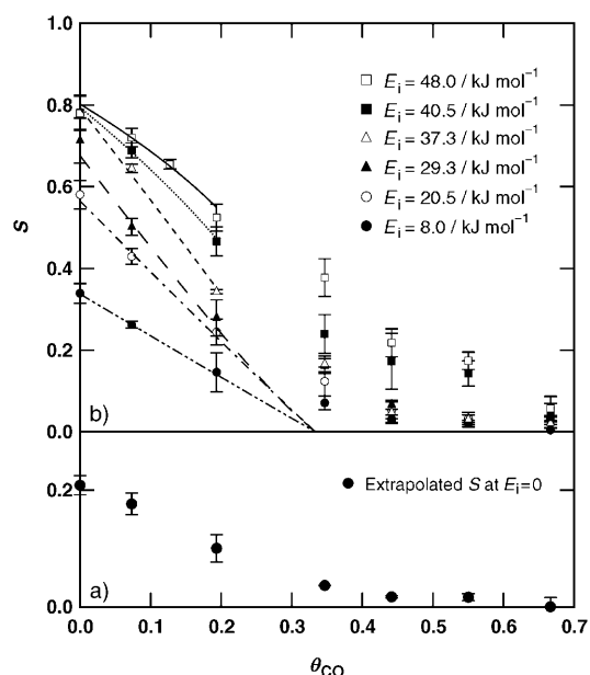
Figure 2. a) The values of S after extrapolation to zero kinetic energy, as a function of \theta_{CO} . These values are obtained from linear fits to the data shown in Figure 1 a. b) Dependence of S of D 2 on \theta_{CO} for CO-covered Ru(0001) at six different initial kinetic energies. The lines are fits to the data by using Equation (1).
