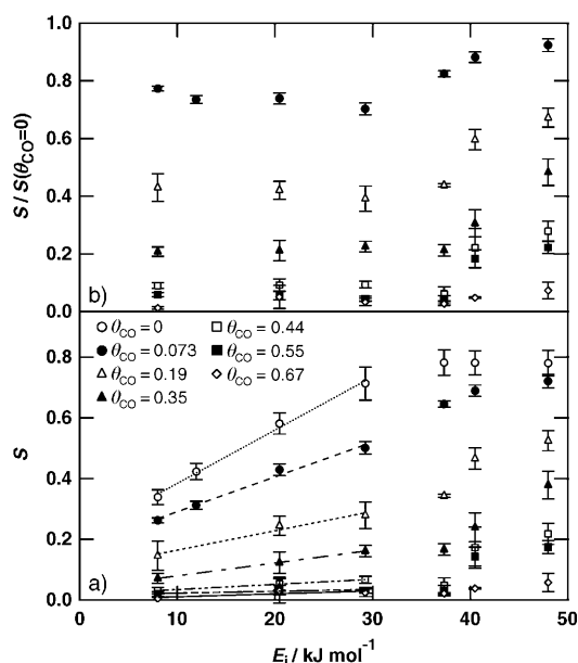
Figure 1. a) Dissociation probability S of D 2 on CO-covered Ru(0001) ( \theta_{CO} = 0 – 2/3 ML) at normal incident angle as a function of D 2 kinetic energy for T_s = 180 K. The lines are obtained by linear fitting of data points for E_i < 30 kJ mol -1 for each S curve in order to extrapolate the value of S to zero kinetic energy. b) The values of S for each \theta_{CO} after normalisation by the corresponding S for bare Ru(0001) as a function of D 2 kinetic energy.
