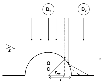
Figure 4. Schematic diagram of the hard-hemisphere collision model. D 2 is treated as a point particle (shown in two positions as circles) and CO is regarded as a hemisphere.
