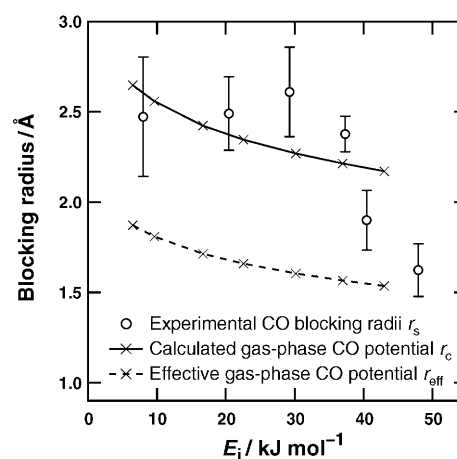
Figure 3. Plot of the radii of \Sigma_{\text{CO}} as a function of D 2 kinetic energy. These values are obtained from fitting Equation (1) to the data shown in Figure 2 for the appropriate coverage region ( \theta_{\text{CO}} < 0.2 ML). The error bars represent estimated standard deviations in the blocking radii. The solid line with crosses gives the maximum radius r_c of the gas-phase H 2 -CO interaction potential contour at each energy. The dashed line with crosses gives r_c/\sqrt{2} , which in the hard-hemisphere model is the radius below which D 2 molecules would be scattered away from the surface.
