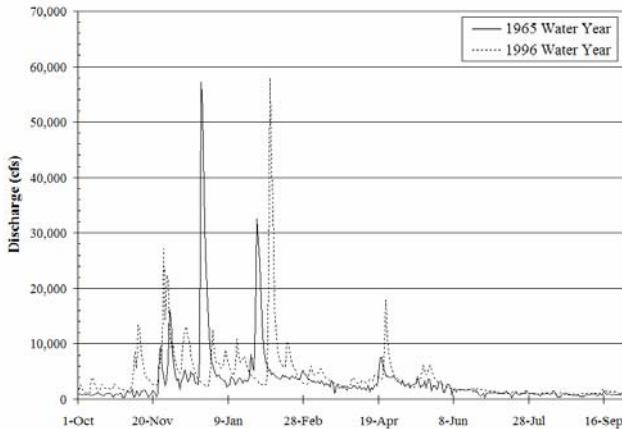
Figure 6. Hydrographs for the Estacada gage (14210000) showing mean daily flow for 1965 and 1996 water years.
