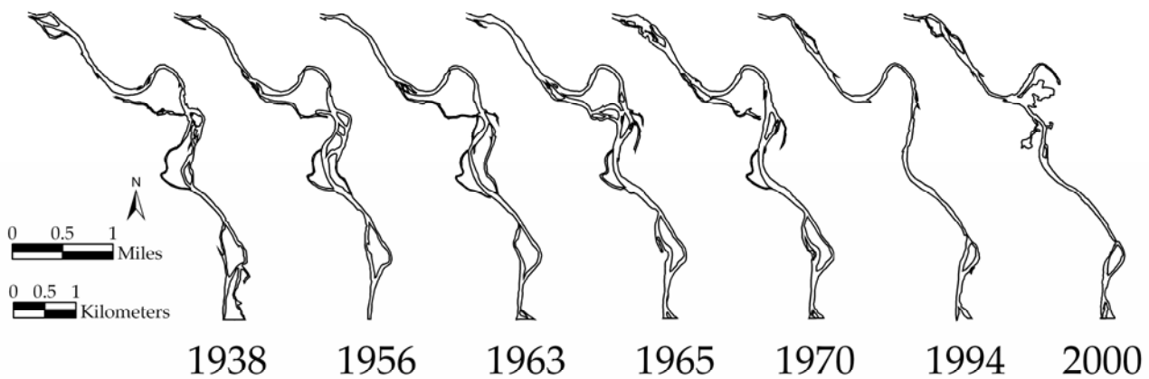
Figure 3. Historic channel plan form changes in River Island reach 1938-2000, based on aerial photos.
