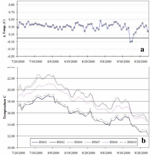
Figure 14. a. Change in temperature between the upstream and downstream probes. b. Average daily temperature data from six recorders during 2000.
