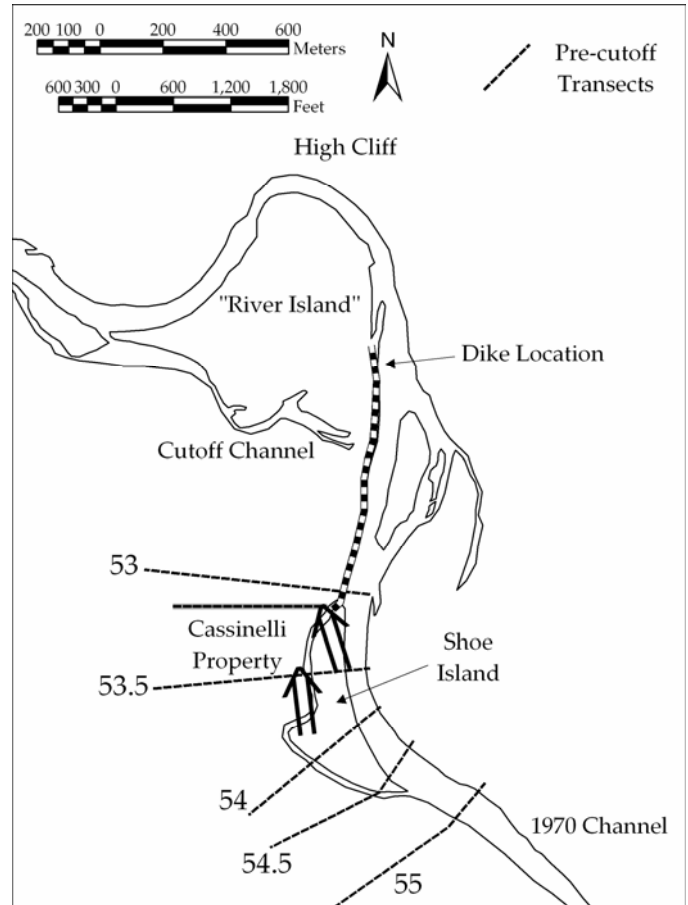
Figure 8. Flood routing map. Bold arrows indicate possible flood entry paths. Numbers refer to Section ID #'s found in Table 2.
