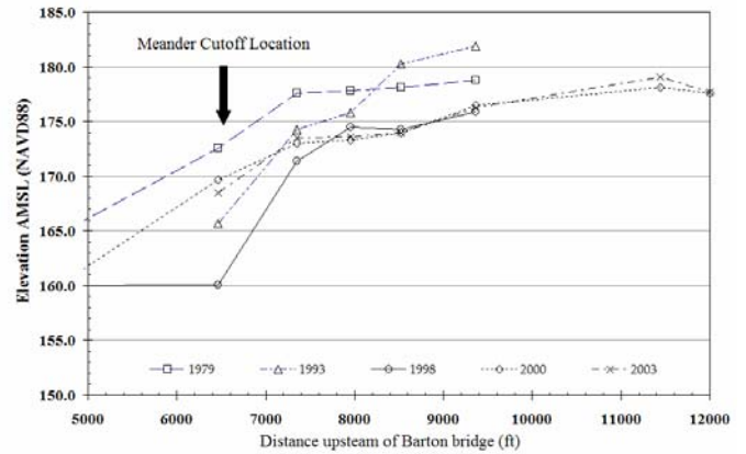
Figure 11. Changes in channel gradient 1979 to 2003 based on thalweg elevations from surveyed transects.
