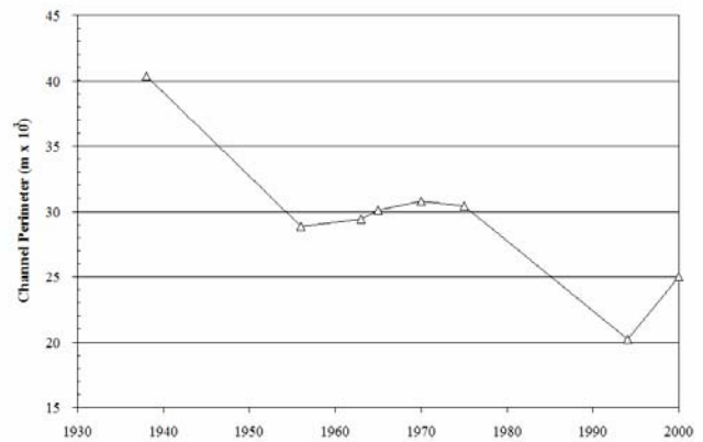
Figure 12. Changes in channel perimeter from RM 12 and RM 17 based on 1938 to 2000 on aerial photos. Discharge at Estacada during the photo dates ranged from 27 to 91 cms (960 to 3,220 cfs).
