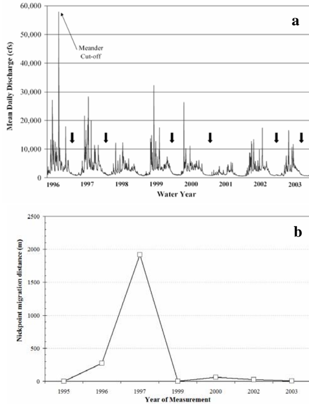
Figure 10. a. Mean daily discharge at Estacada (1421000) 1996-2003. b. Knick point migration distance measured upstream of Barton Bridge during the same time period. Arrows indicate approximate timing of knick point measurements from photos and ground survey measurements.
