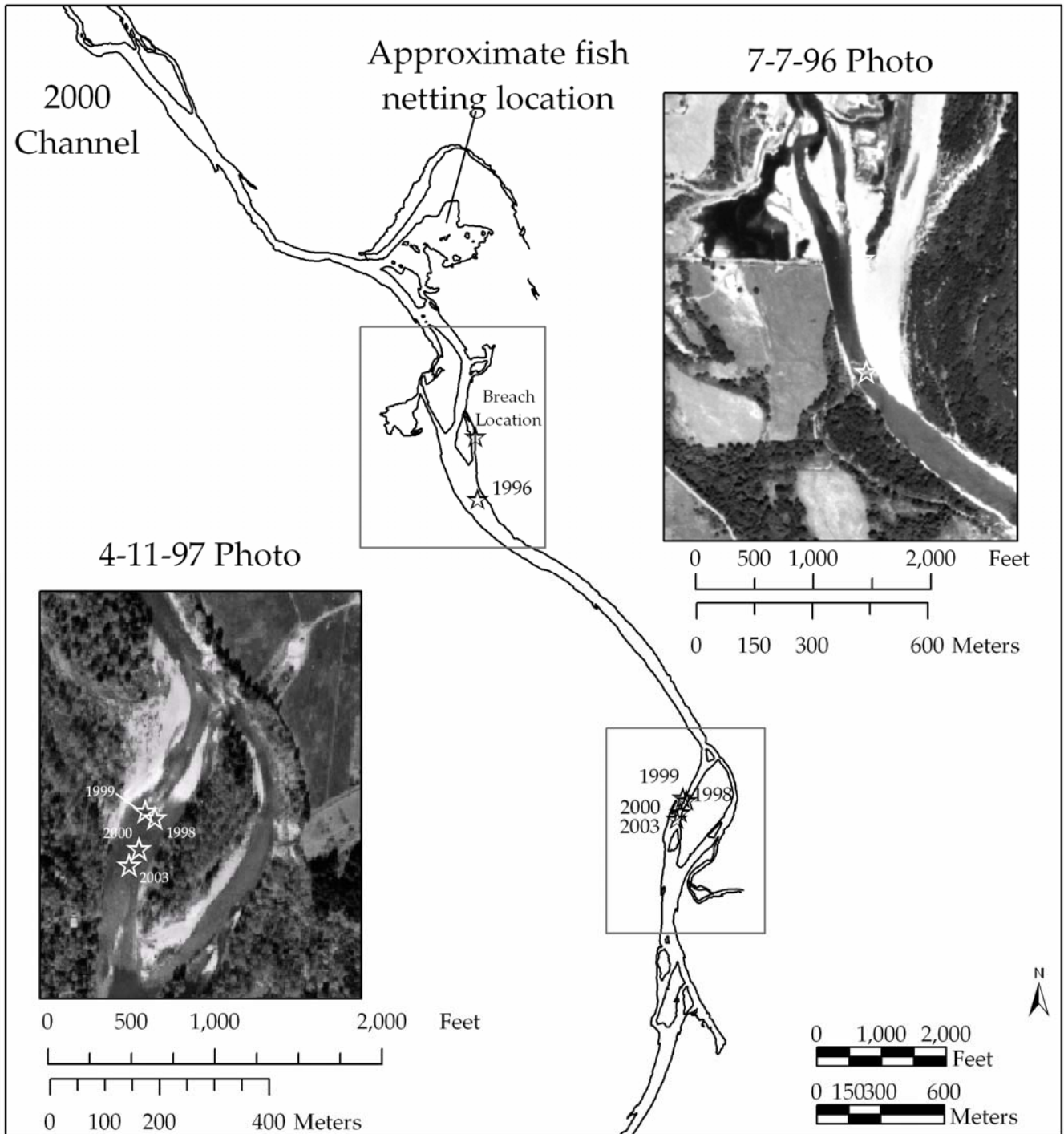
Figure 9. Knick point migration between 1996 and 2003. Note the location of fish netting in the northern pit. Stars indicate a measured knick point locations.
