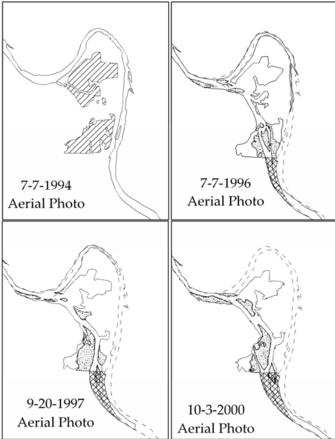
Figure 13. Erosion and deposition patterns in the River Island reach 1996-2000. The 1994 channel is shown with a dashed line for reference. Solid lines show the post-1994 channel configuration. Stippled regions are exposed gravel bars. Cross-hatched area is eroded river bank upstream of the cutoff. Hachured area represents the pre-cutoff pond area.
