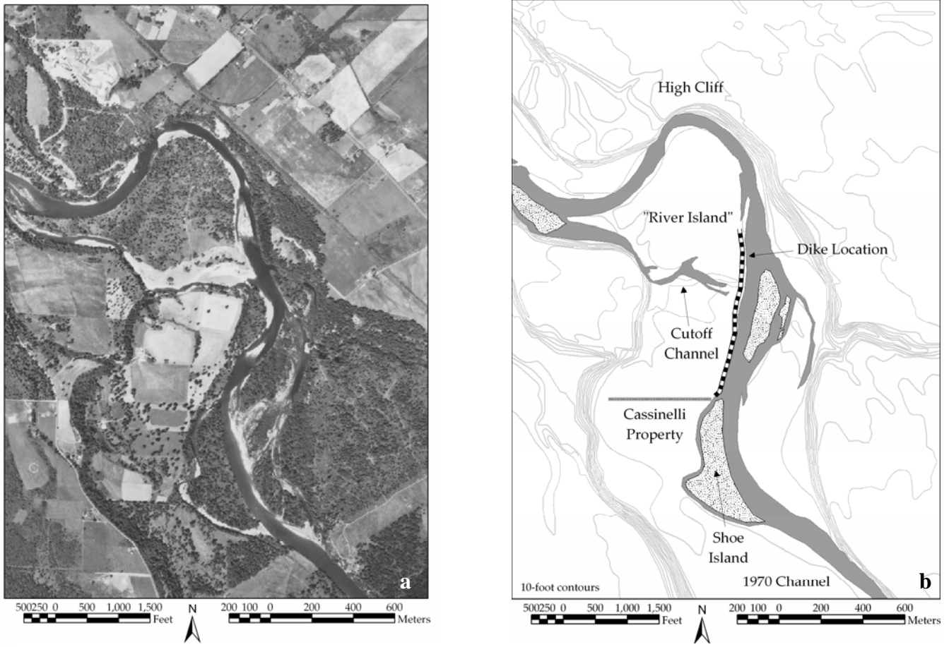
Figure 5. a. Aerial photo taken June 17, 1963. b. Detailed site map showing the configuration of the site after dike construction.
